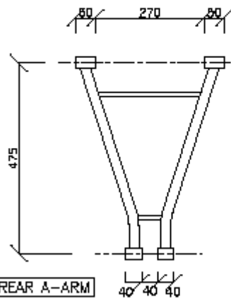
REAR SUSPENSION CONFIGURATION
