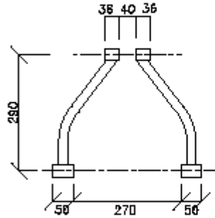
UPPER REAR SUSPENSION ARMS (TWO)
