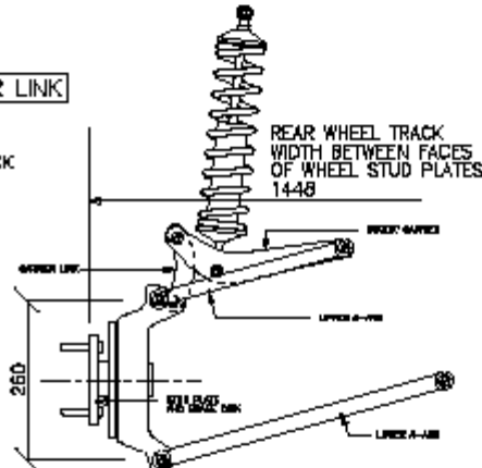
REAR SUSPENSION CONFIGURATION
