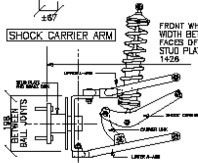
FRONT SUSPENSION CONFIGURATION
