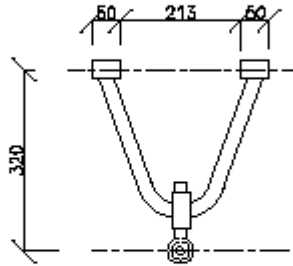
UPPER FRONT A-ARM
