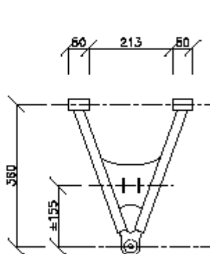
LOWER FRONT A-ARM
